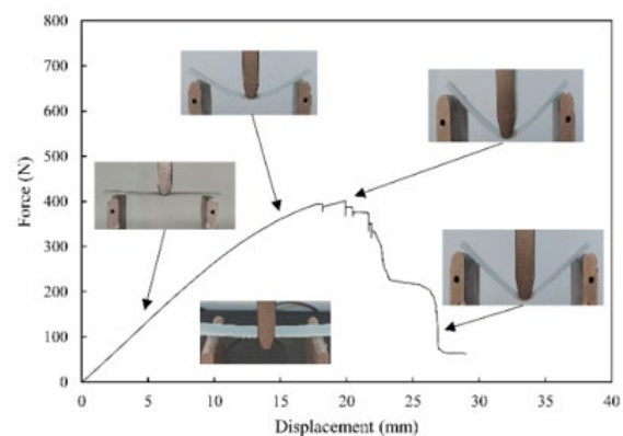
Fig. 9. Specimen VPC-1 during flexure test
