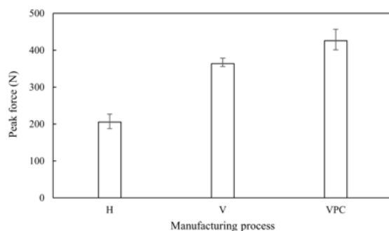
Fig. 8. Nominal values of peak forces according to manufacturing process
