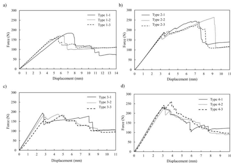
Fig. 5. Force displacement graph of a) Type 1, b) Type 2, c) Type 3 and d) Type 4
