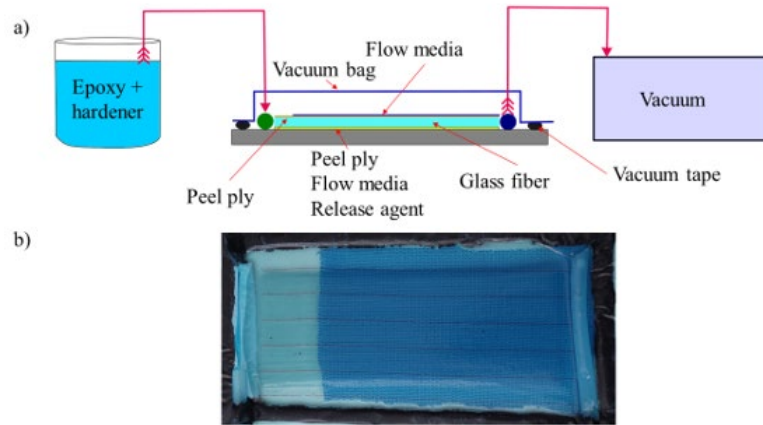
Fig. 4. a) Diagram of vacuum infusion process, b) top view of sample
