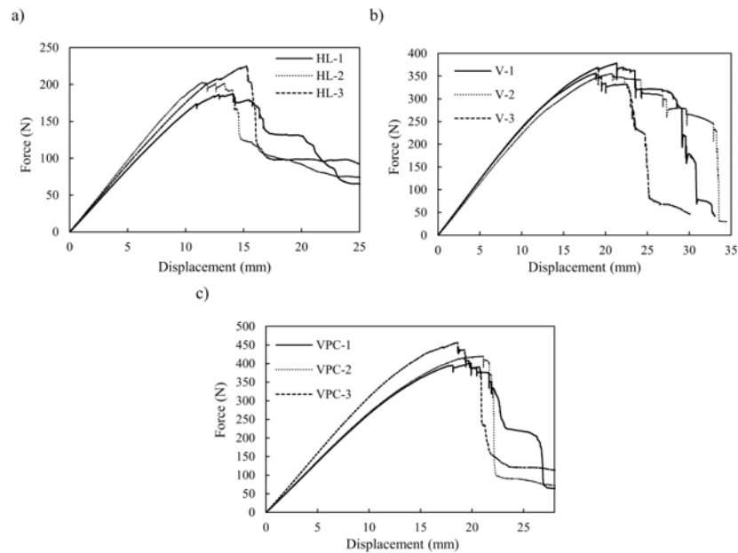
Fig. 7. Results ([4G]s) of hand lay-up (HL), vacuum infusion (V), cured flat samples (VPC)
