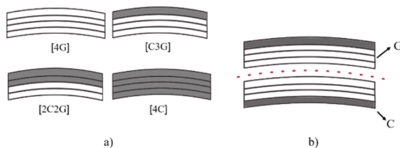
Fig. 2. a) Sequences of fiber layers applied in the study, b) illustration of symmetry plane
