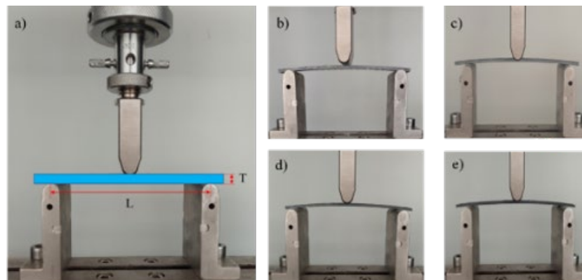
Fig. 3. Three-point flexure test a) [4G]s, b) [C3G]s, c) [2C2G]s, d) [4C]s
