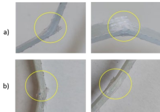
Fig. 10. Sample photographs of a) V and b) VPC after flexural test
