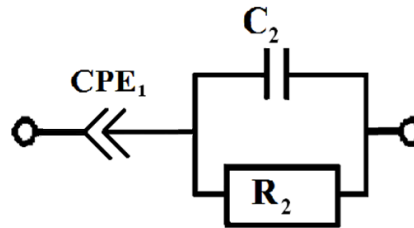
Fig. 3. Equivalent circuit for modeling impedance spectra of PEO/OMMT nanocomposites.
