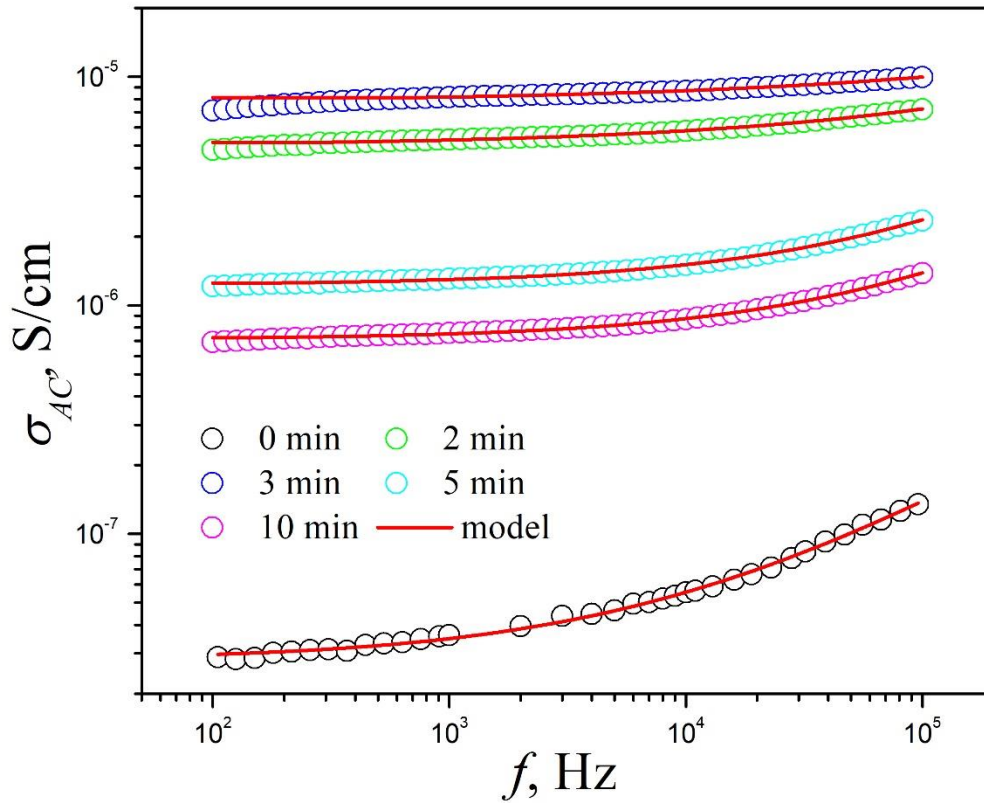
Fig. 1. Frequency dependence curves of electrical conductivity at alternating current for PEO/OMMT nanocomposites produced using different mixing times. Solid line is Jonscher model (Eq. 1).
