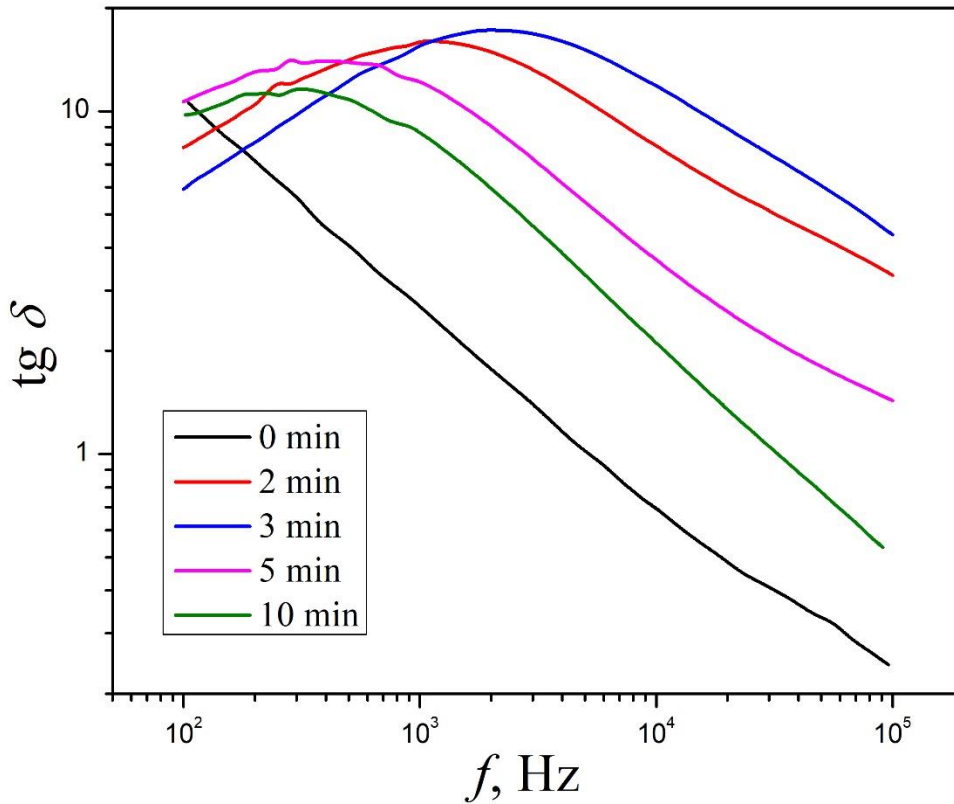
Fig. 4. Frequency dependences of dielectric loss tangent of PEO/OMMT nanocomposites.
