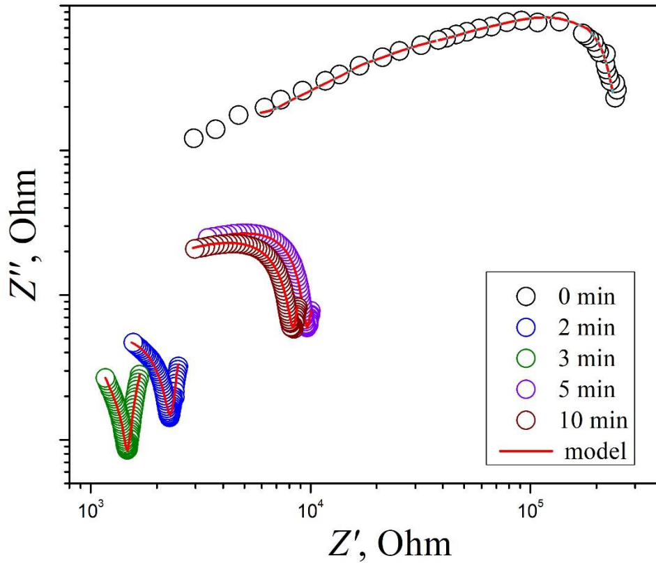
Fig. 2. Nyquist plots of PEO/OMMT nanocomposites for different mixing times. Solid lines display fitting using an equivalent circuit.
