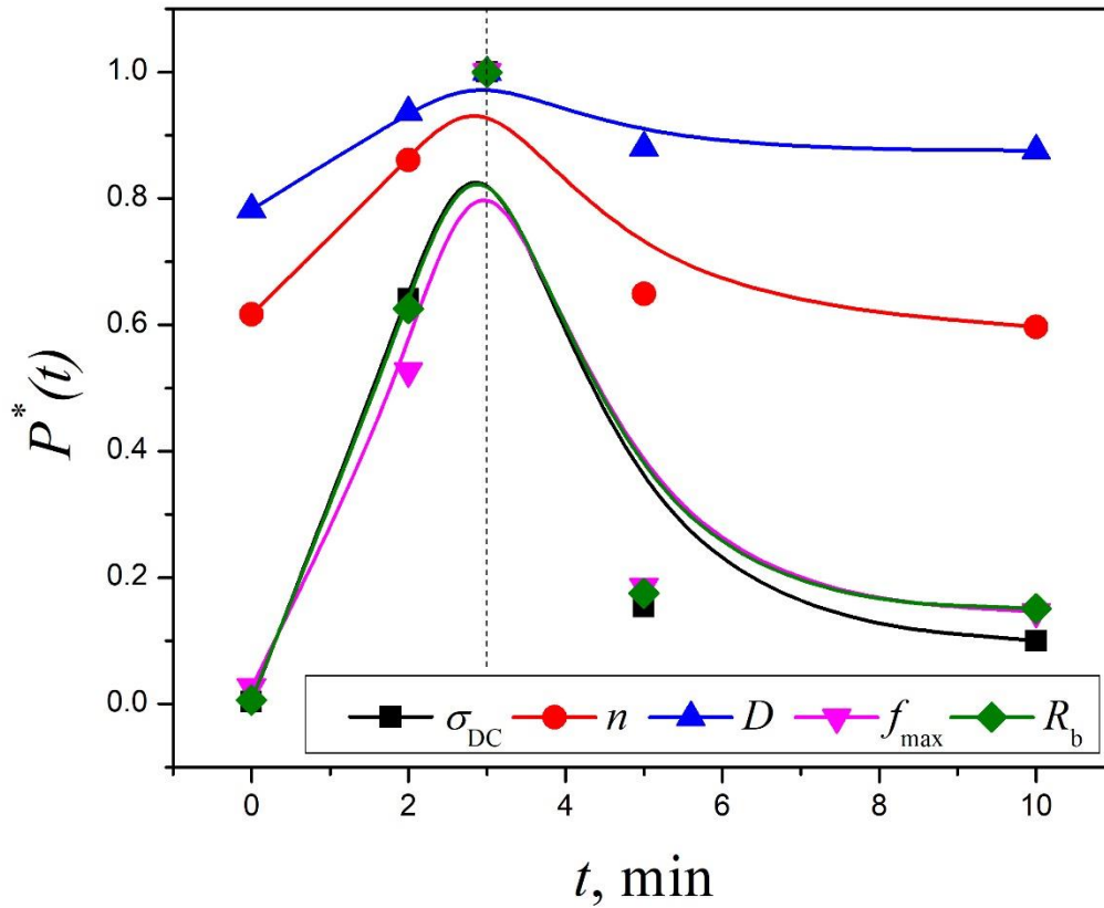
Fig. 5. Electrical and dielectric characteristics of PEO/OMMT nanocomposites in normalized coordinates as a function of mixing time.
