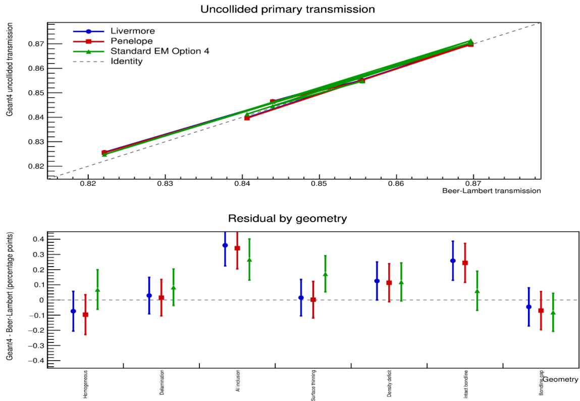
Figure 6. Comparison of Geant4 uncollided-primary transmission with the Beer-Lambert prediction for seven modelled configurations and three electromagnetic physics constructors. Upper panel presents the identity comparison, whereas the lower panel shows the signed Geant4-minus-analytical residual in percentage points. Monte Carlo error bars represent binomial standard uncertainties from runs containing 4 \times 10^6 incident histories each.
