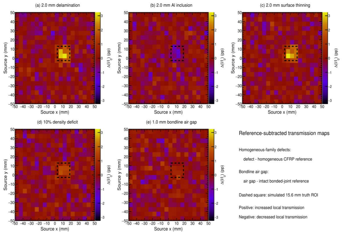
Figure 3. Defect-minus-matched-reference transmission maps. Delamination, thinning, density deficit, and bond-line gap increase transmission; aluminium produces the opposite sign. Common matched-reference rule is used within each physical panel family.
