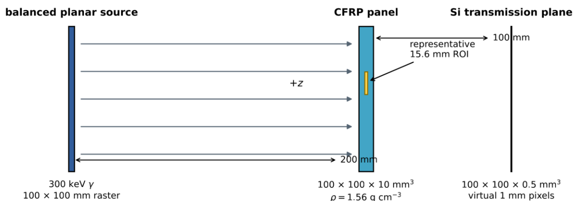
Figure 1. Normal-incidence single-projection geometry. Balanced planar raster emits equal histories into each 1 \times 1 mm 2 source pixel. The highlighted region shows the common 15.6 \times 15.6 mm 2 final-defect footprint; its through-thickness material depends on the defect class.
