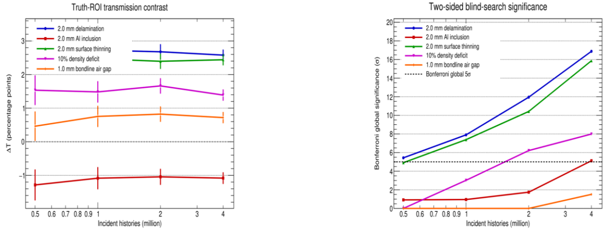
Figure 5. (a) Signed known-ROI contrast. (b) Bonferroni-corrected blind significance. Exposure dependence was obtained from nested prefixes of locked simulation runs. Points at different exposure levels are therefore not independent repetitions. The dashed line in panel (b) indicates the global 5\sigma detection threshold. First stable tested crossing is marked directly on each successful curve: 0.5, 1, 2, and 4 million histories for delamination, surface thinning, density deficit, and aluminium inclusion, respectively; bond-line gap did not reach the threshold.
