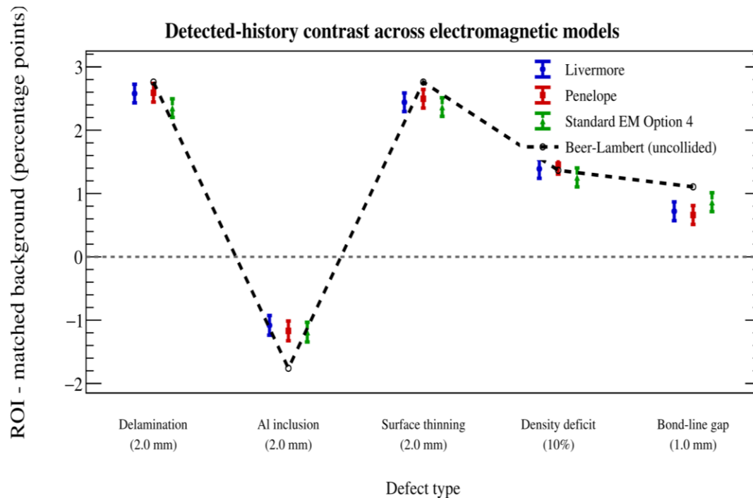
Figure 7. Detected-history ROI contrasts for five defect classes obtained with Livermore, Penelope, and Standard EM Option 4 constructors, together with corresponding uncollided Beer–Lambert predictions. Monte Carlo error bars show propagated binomial standard uncertainties. Horizontal marker offsets are used only for visual separation, and dashed analytical curve is a guide to the eye. Exact agreement with the analytical curve is not expected because the two quantities employ different transmitted-history definitions.
