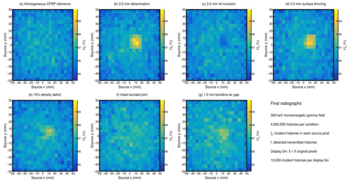
Figure 2. Four-million-history source-normalized transmission radiographs for two references and five locked defect cases. Demonstration rebinning preserves incident and detected count totals.
