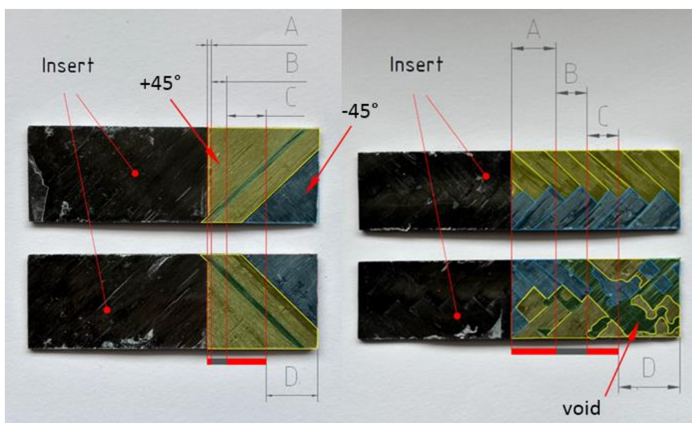
Figure 15. Visual assessment of fracture surfaces of specimens DCB-1 (left) and DCB-5 (right).
