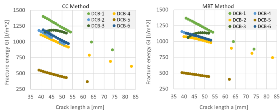
Figure 12. Fracture toughness G_I evolution as a function of crack length for all DCB test specimens determined by CC (left) and MBT methods (right).
