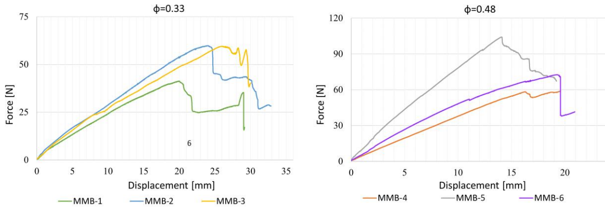
Figure 19. Load-displacement curve for \phi=0.33 mixity specimens (left), \phi=0.48 mixity (right).
