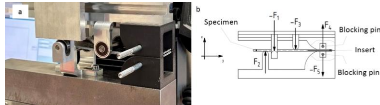
Figure 5. MMB specimen loading conditions.
