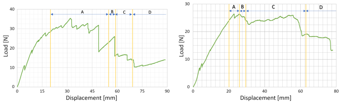
Figure 16. Load–displacement curves corresponding to visual assessment of specimens DCB-1 (left) and DCB-1 (right).
