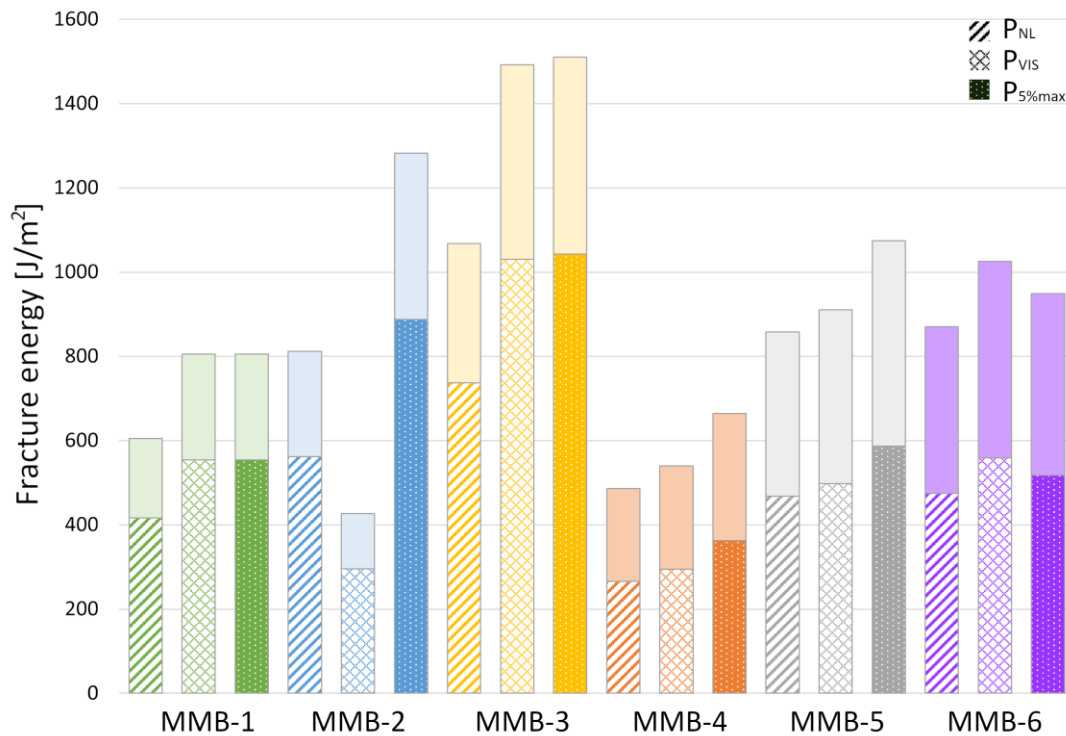
Figure 20. P_{NL} , P_{VIS} , P_{5\%max} fracture energy for all MMB specimens.
