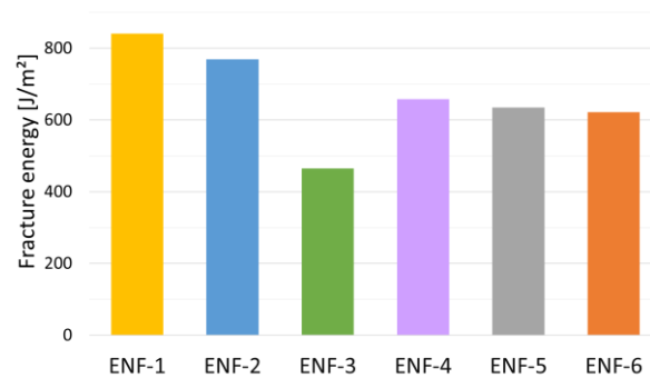
Figure 18. Fracture energy G_{IIc} for all ENF specimens
