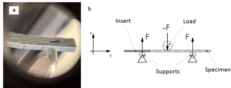
Figure 4. Mode II a) layer displacement at end of test b) ENF method diagram.
