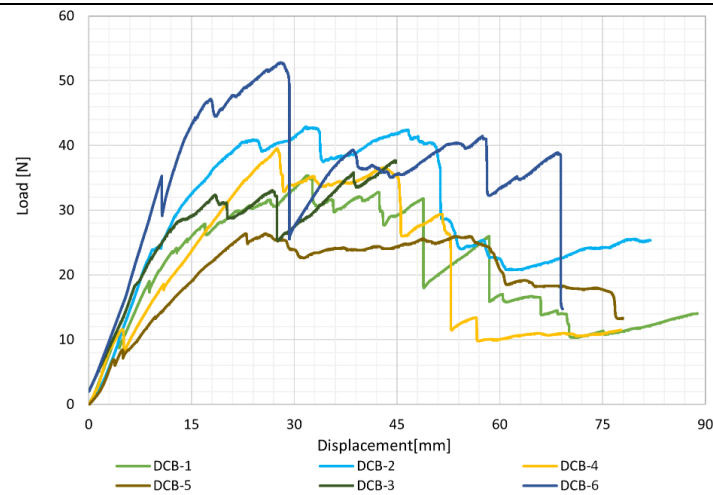
Figure 13. Load–displacement curves for all DCB specimens.
