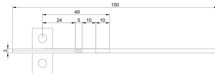
Figure 8. MMB specimen with positions of markers.
