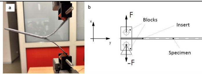
Figure 3. Mode I testing a) specimen at end of test b) DBC method diagram.
