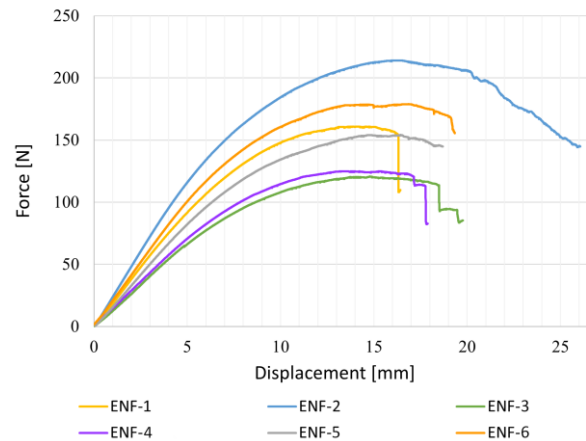
Figure 17. Load–displacement curves for all ENF specimens.
