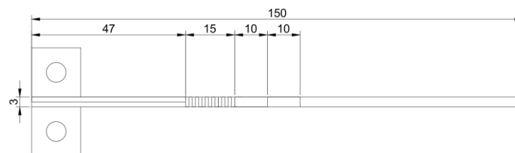
Figure 6. Position of markers on DCB specimen.
