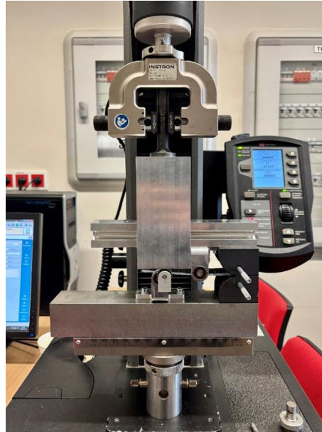
Figure 11. MMB test setup.
